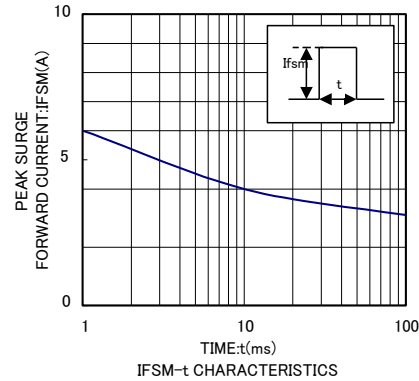
IFSM-t CHARACTERISTICS
