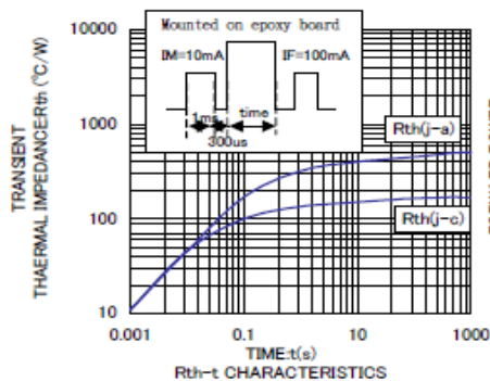
Rth-t CHARACTERISTICS
