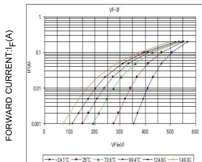
Fig. 1 Forward characteristics
