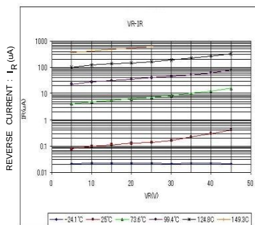
Fig. 2 Reverse characteristics
